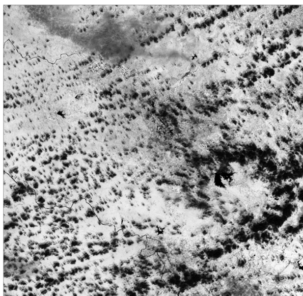
NDVI Sentinel-2
